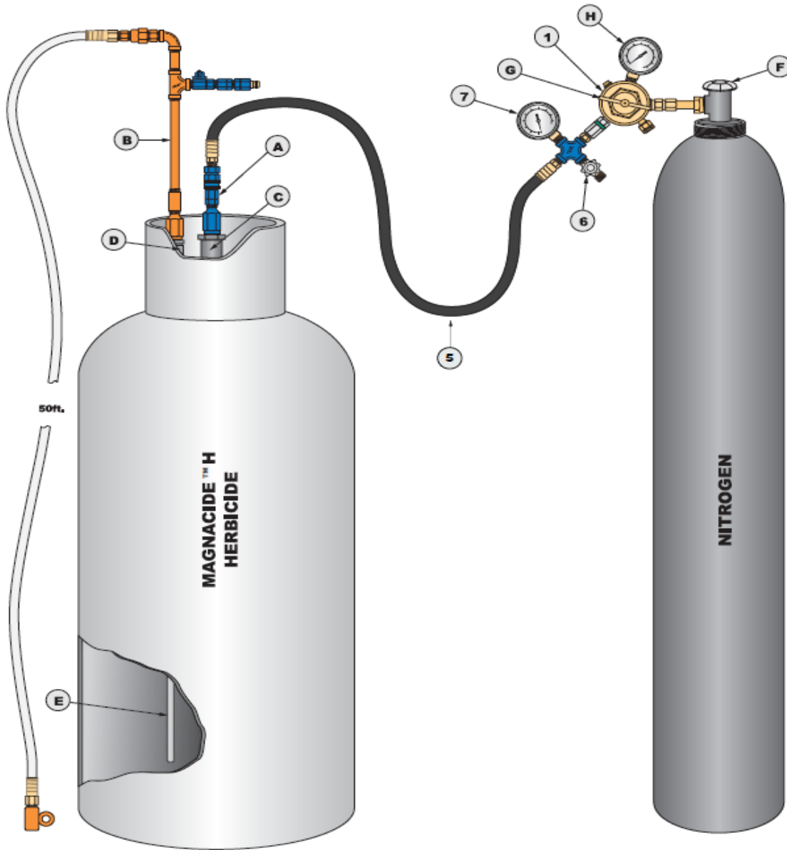
Figure 1. MAGNACIDE H Herbicide Application Set Up
